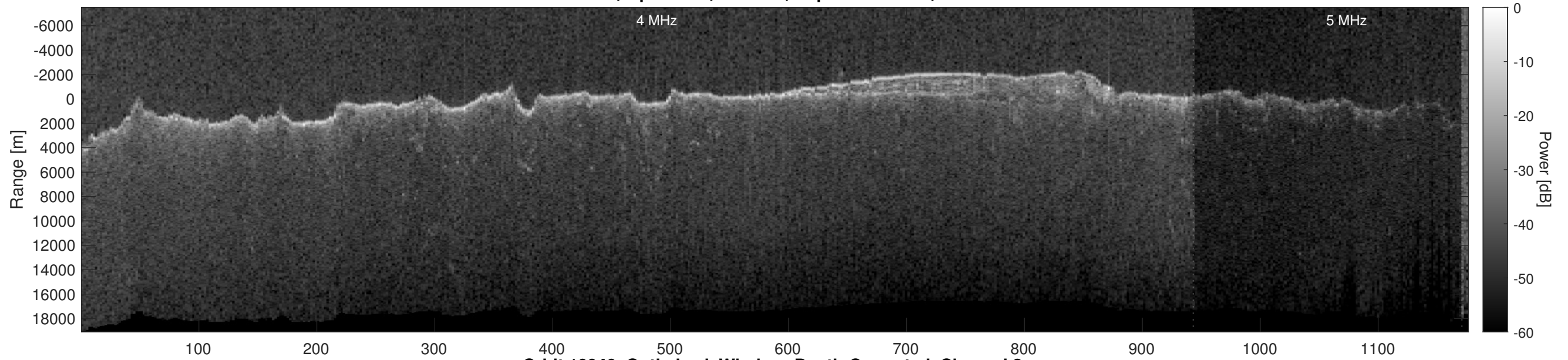
Orbit 10940, Optimized, Window, Depth-Corrected, Channel 2
