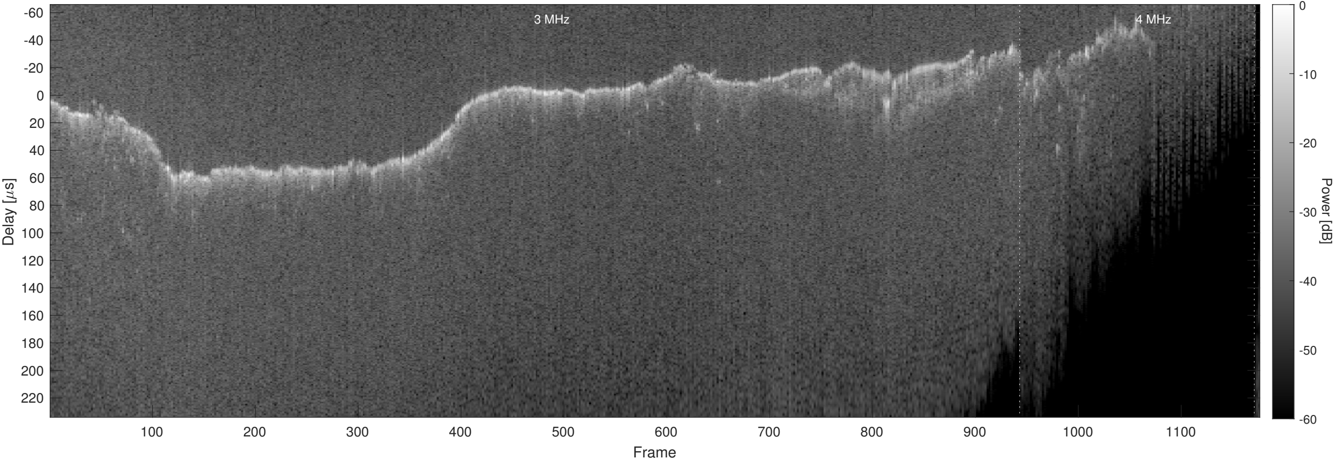
Orbit 10941, Chapman, No Window, Channel 2
