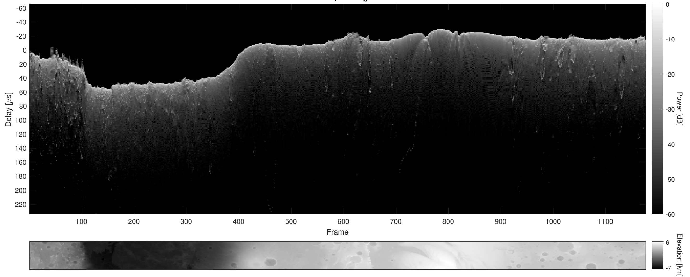
Orbit 10941, Cluttergram
