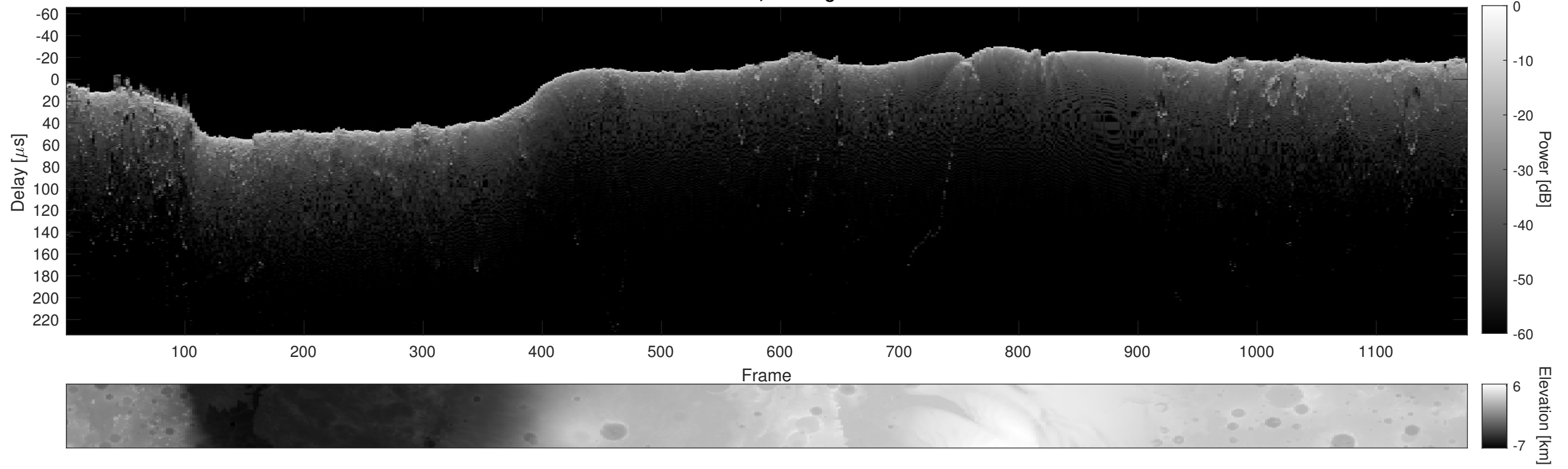
Orbit 10941, Cluttergram
