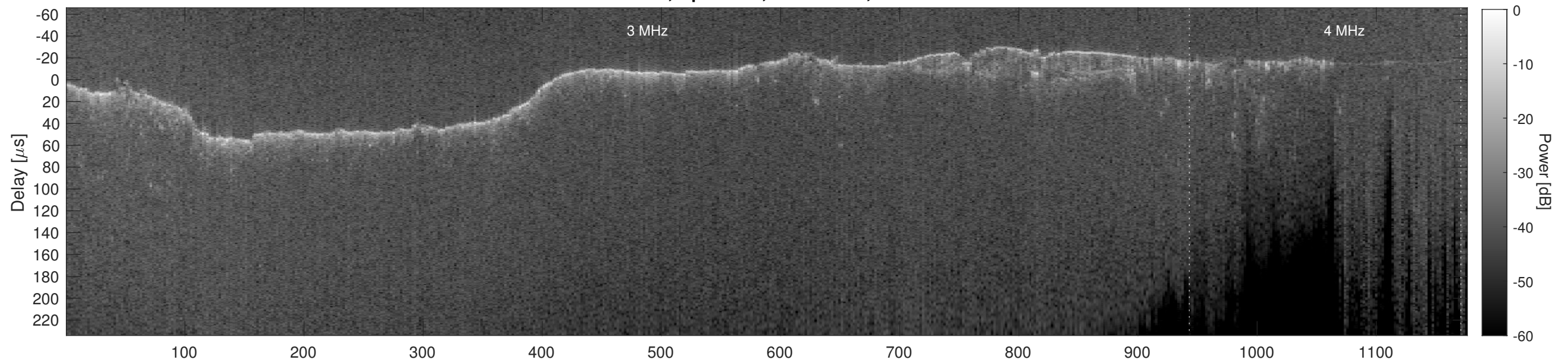
Orbit 10941, Cluttergram
