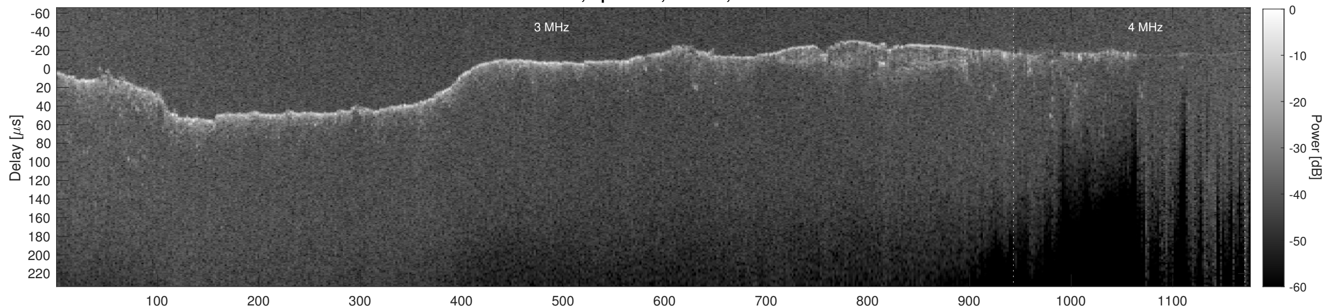
Orbit 10941, Cluttergram
