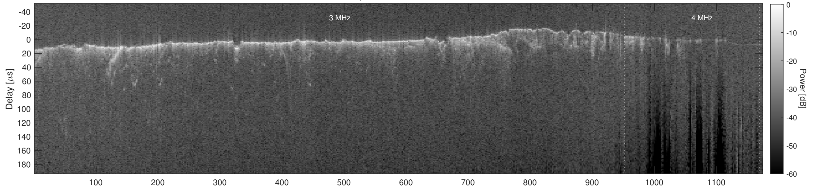
Orbit 10945, Cluttergram
