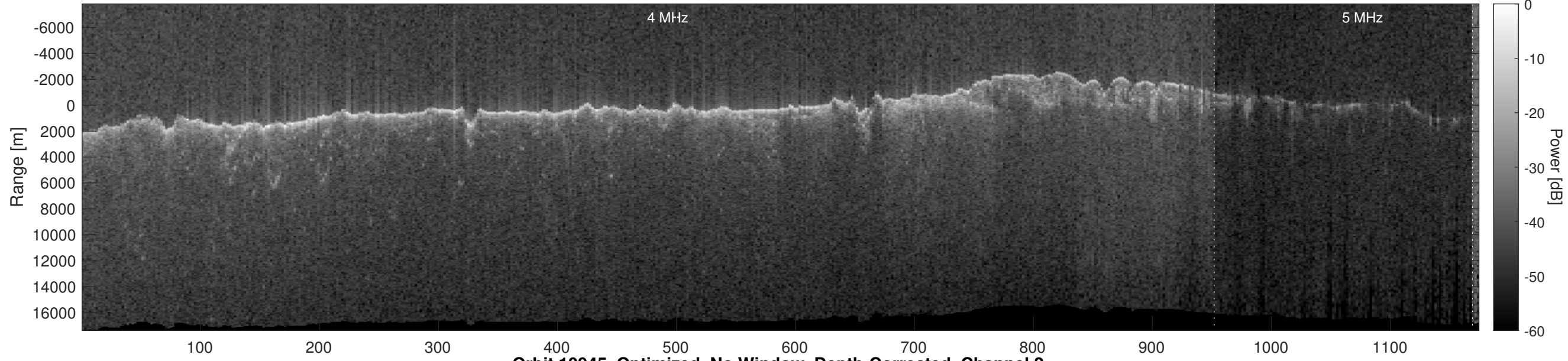
Orbit 10945, Optimized, No Window, Depth-Corrected, Channel 2
