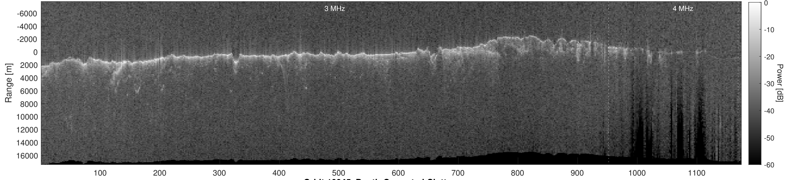
Orbit 10945, Depth-Corrected Cluttergram
