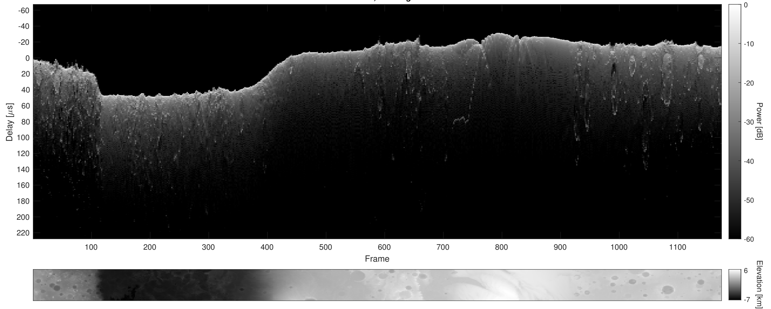
Orbit 10948, Cluttergram
