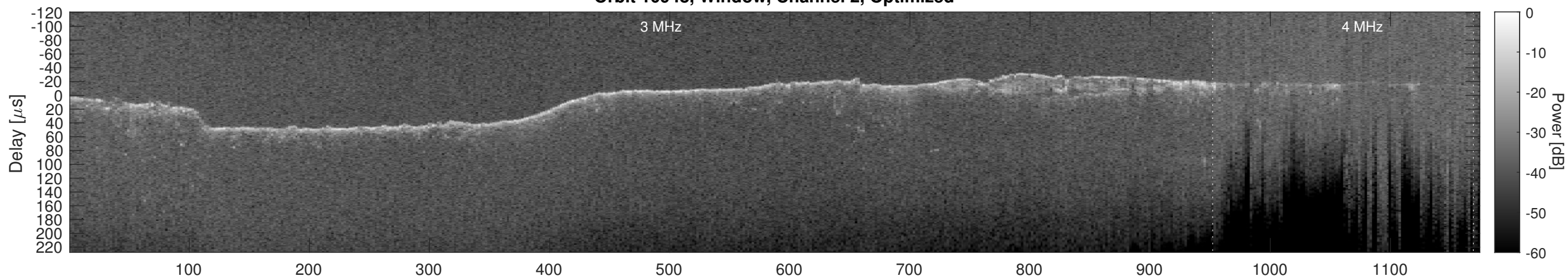
Orbit 10948, Cluttergram
