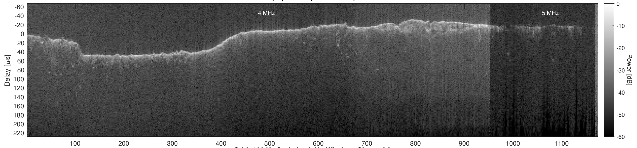
Orbit 10948, Optimized, No Window, Channel 2
