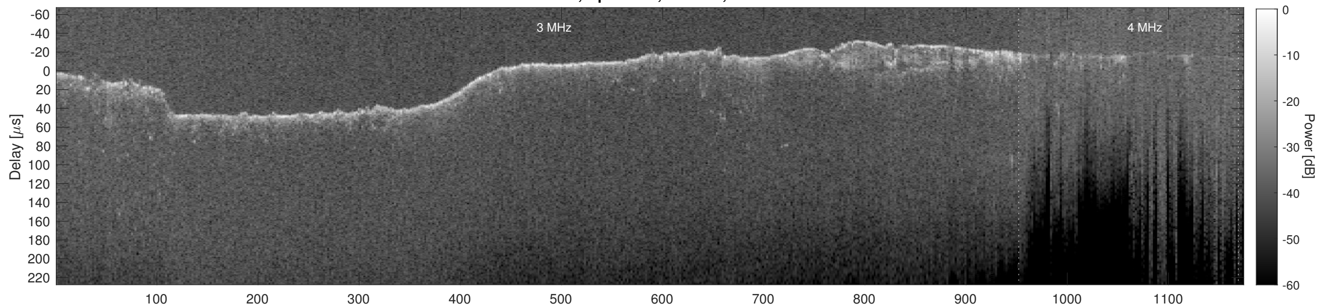
Orbit 10948, Cluttergram
