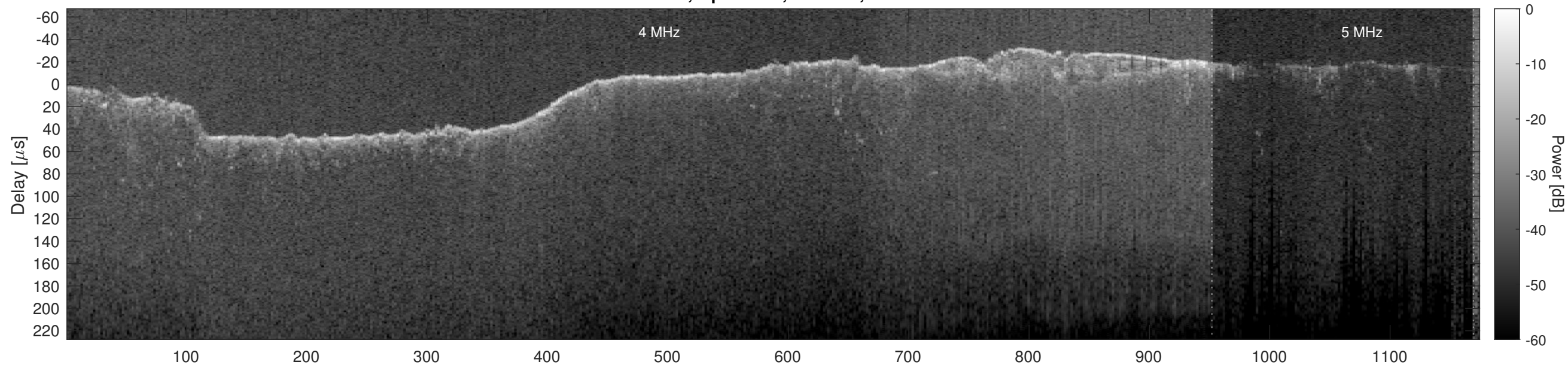
Orbit 10948, Optimized, Window, Channel 2
