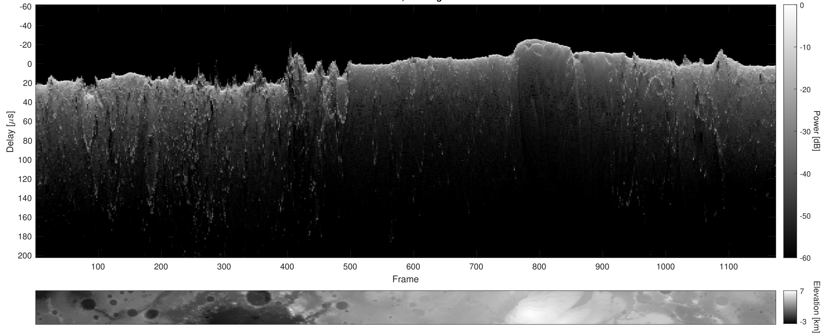
Orbit 10949, Cluttergram
