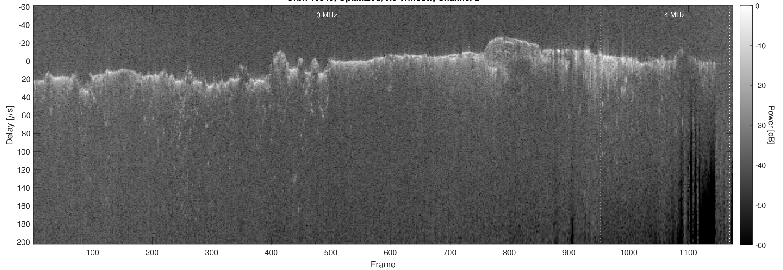
Orbit 10949, Optimized, No Window, Channel 2
