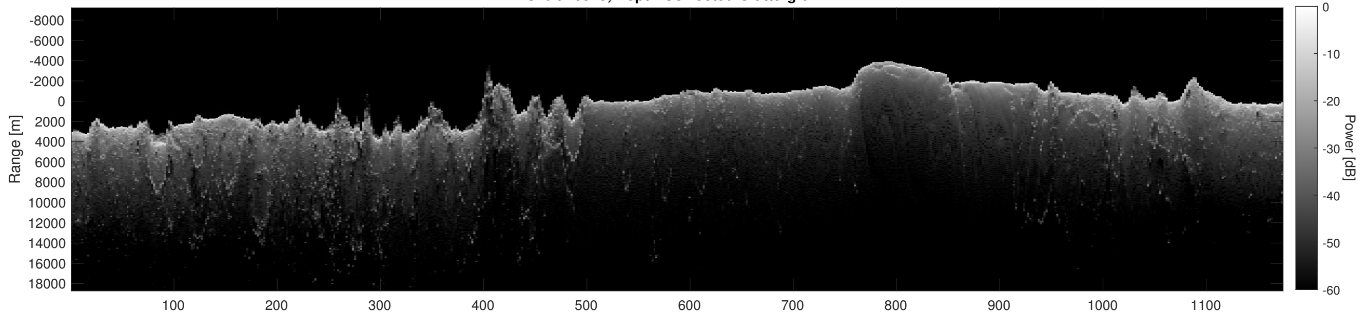
Orbit 10949, Depth-Corrected Cluttergram
