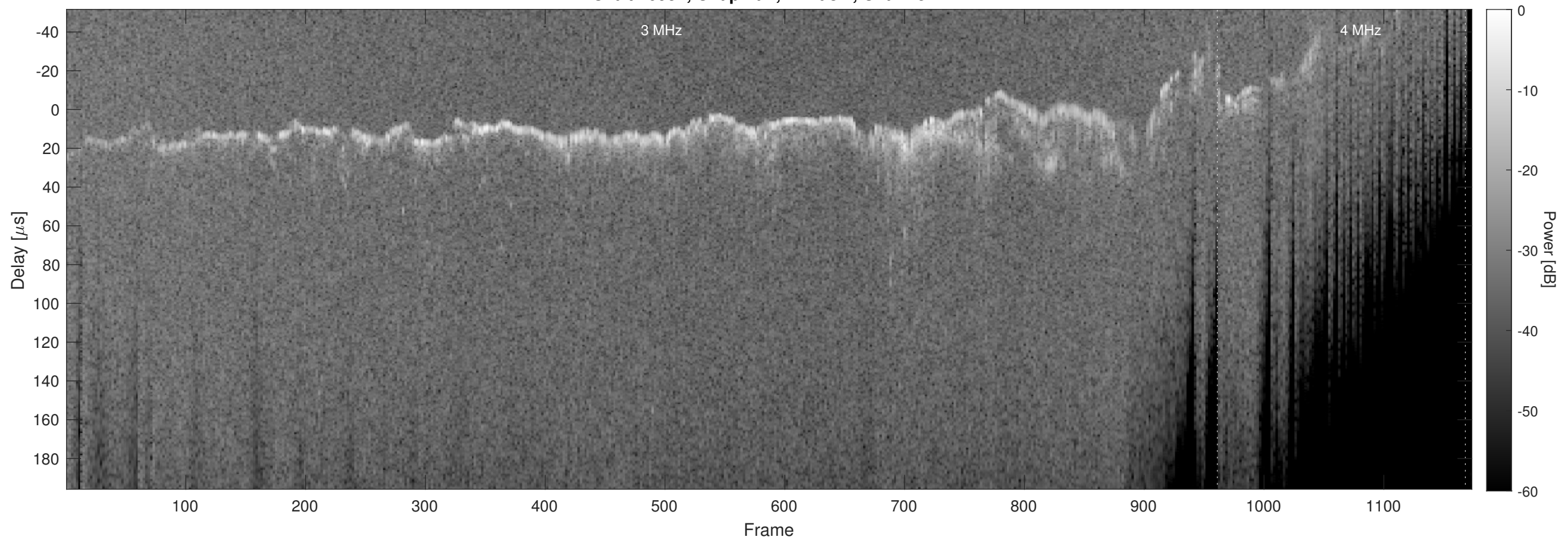
Orbit 10952, Chapman, Window, Channel 2
