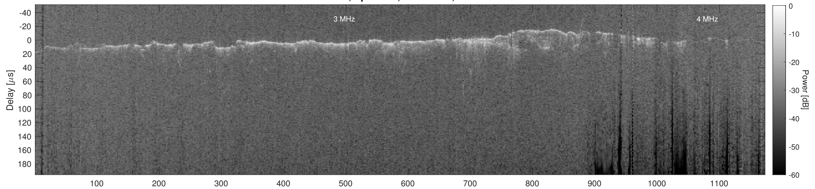
Orbit 10952, Cluttergram
