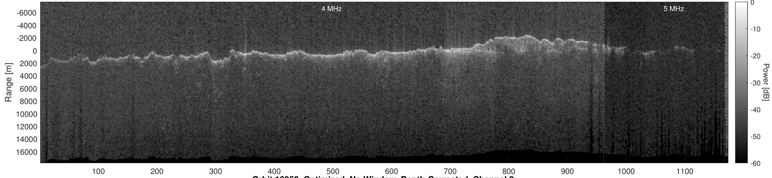
Orbit 10952, Optimized, No Window, Depth-Corrected, Channel 2
