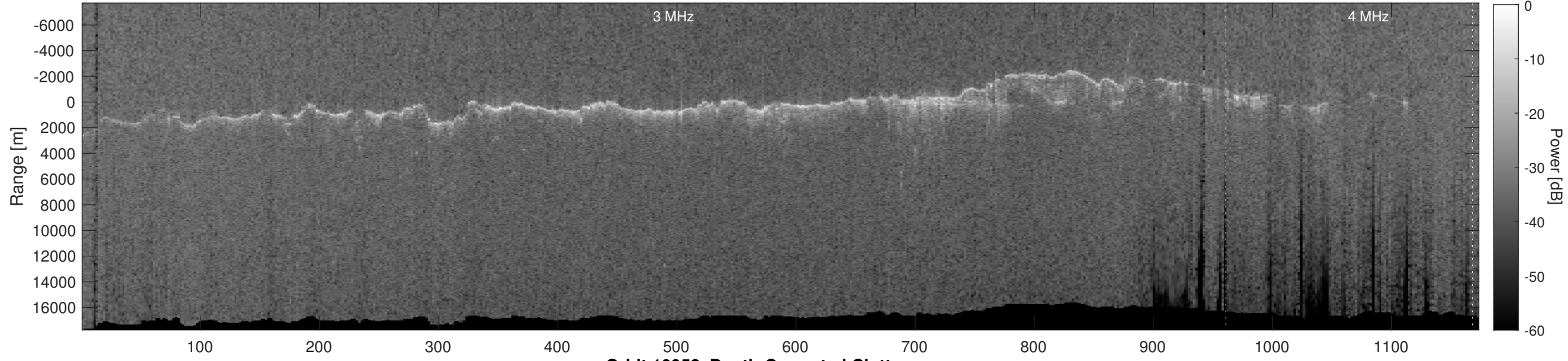
Orbit 10952, Depth-Corrected Cluttergram
