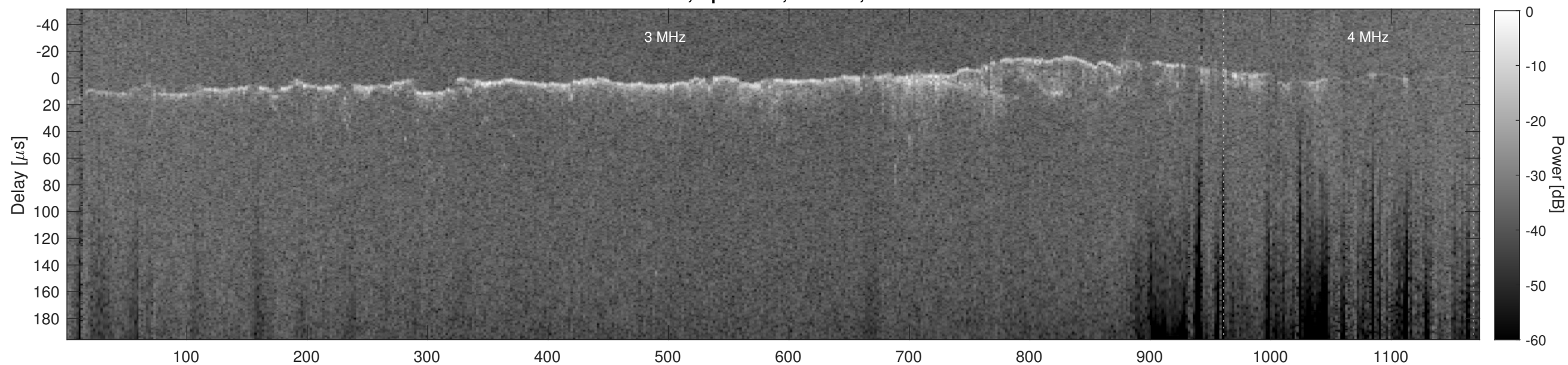
Orbit 10952, Cluttergram
