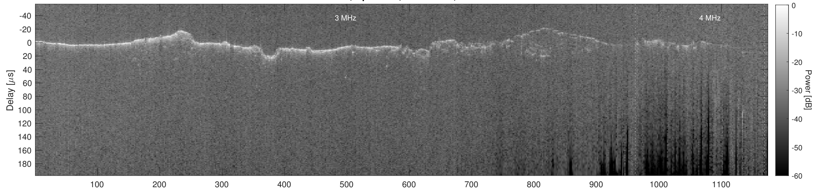
Orbit 10953, Cluttergram
