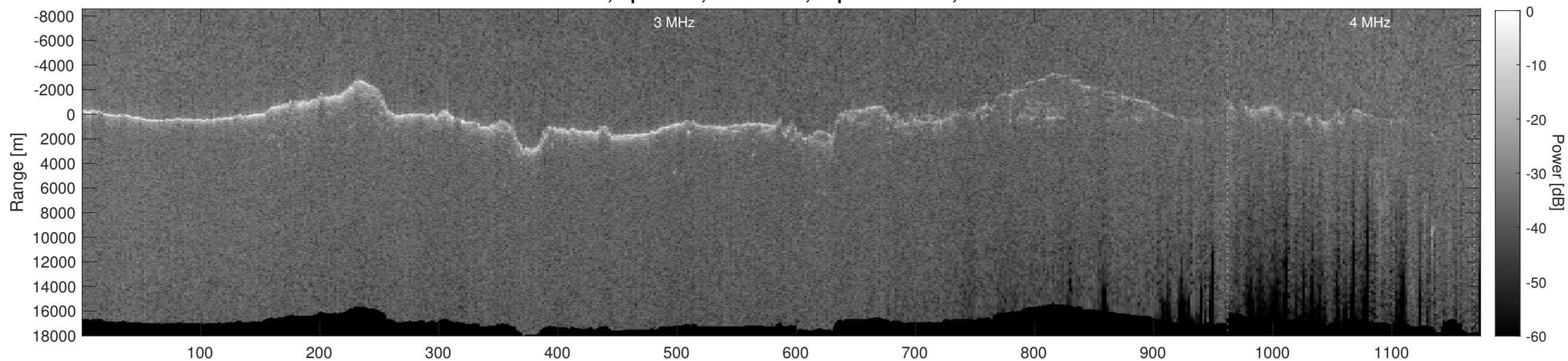
Orbit 10953, Depth-Corrected Cluttergram
