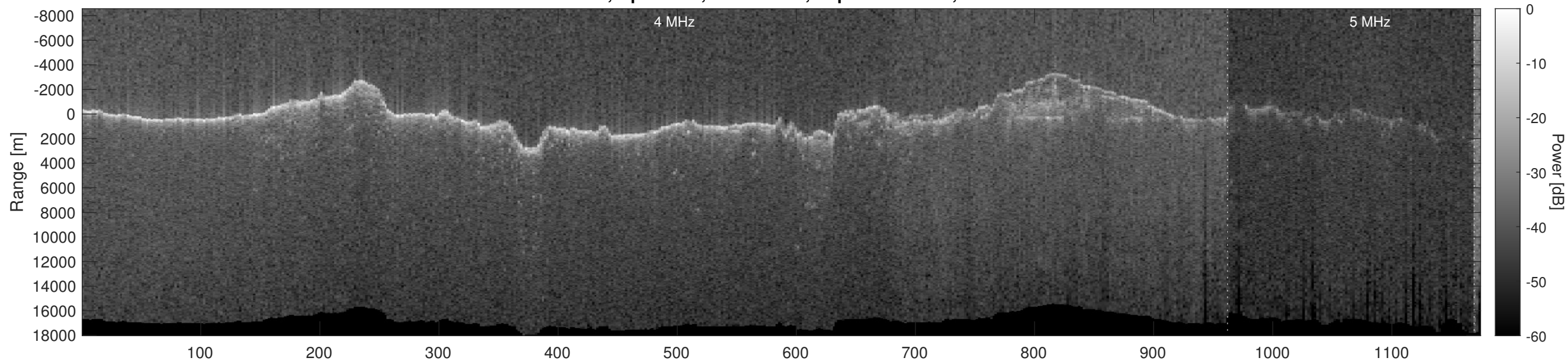
Orbit 10953, Optimized, No Window, Depth-Corrected, Channel 2
