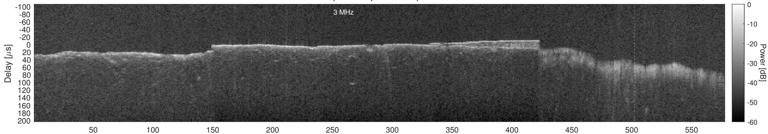
Orbit 10954, Window, Channel 2, Chapman
