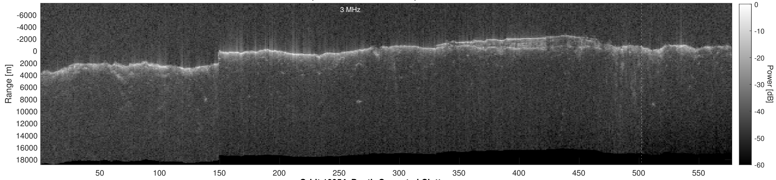
Orbit 10954, Depth-Corrected Cluttergram
