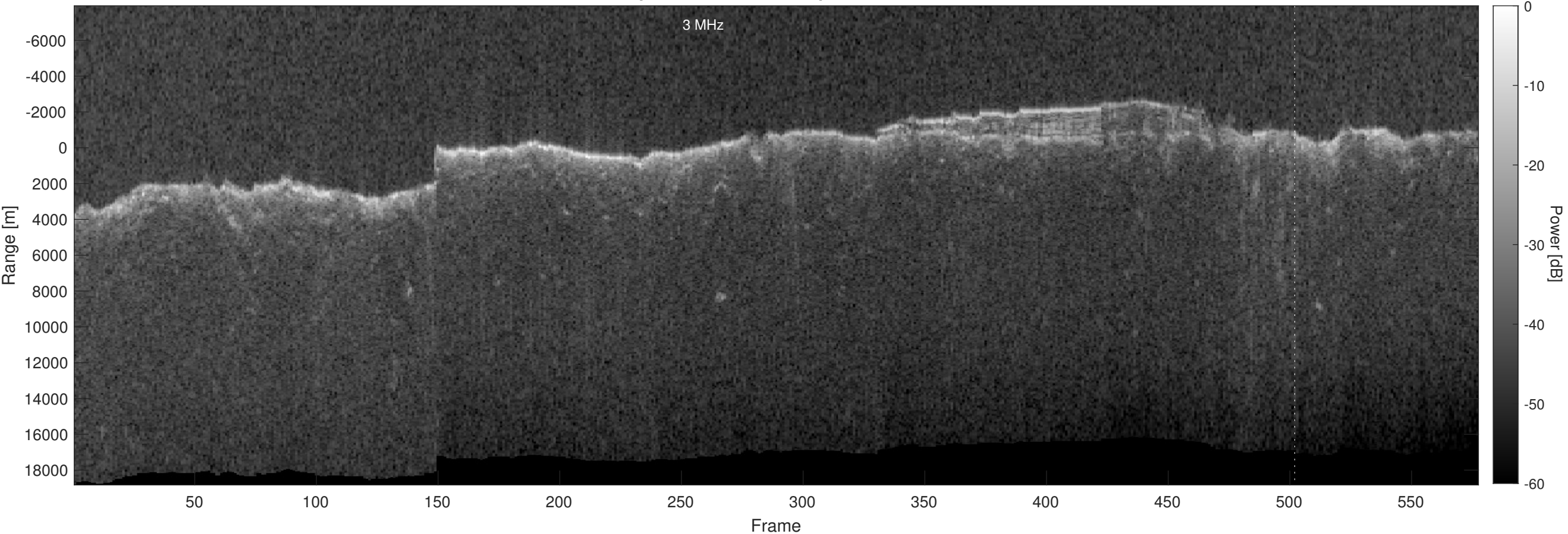
Orbit 10954, Optimized, Window, Depth-Corrected, Channel 2
