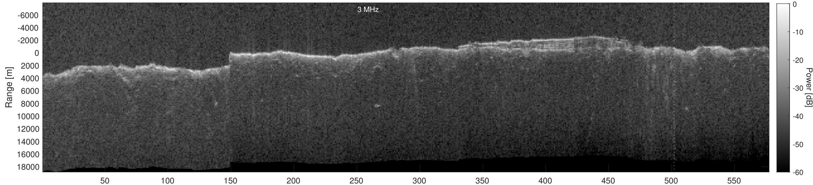
Orbit 10954, Depth-Corrected Cluttergram
