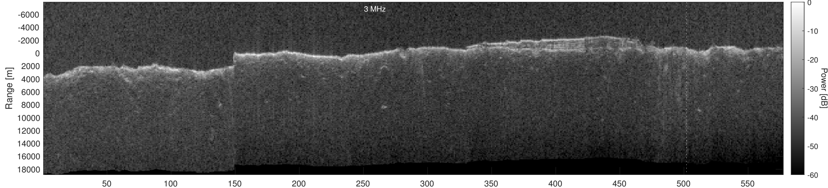
Orbit 10954, Optimized, Window, Depth-Corrected, Channel 2
