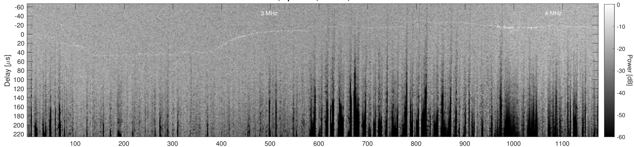
Orbit 10955, Cluttergram
