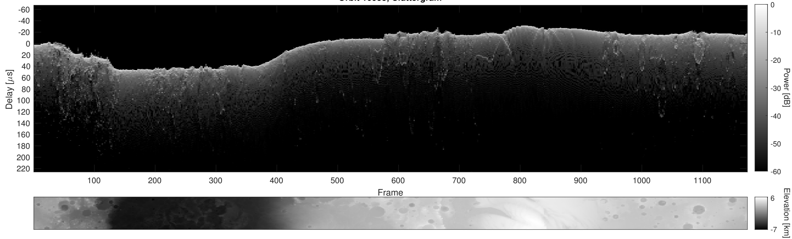
Orbit 10955, Cluttergram
