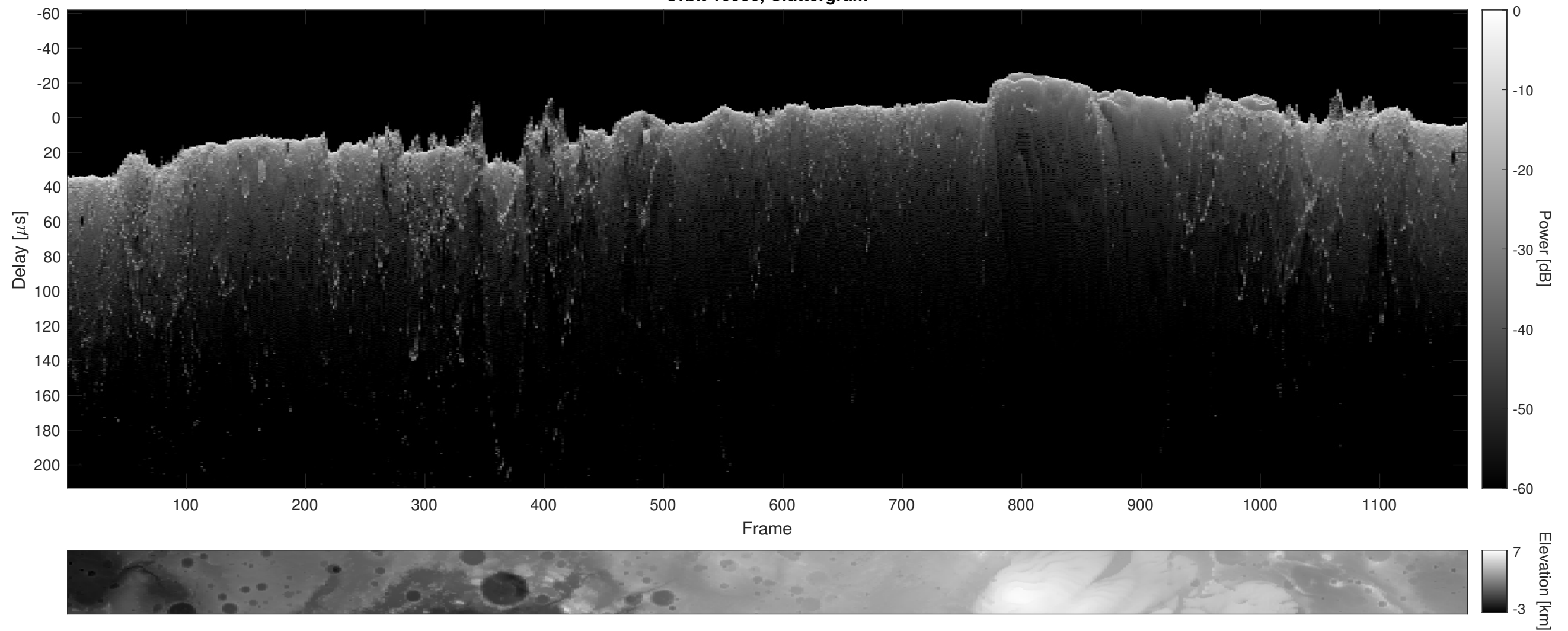
Orbit 10956, Cluttergram
