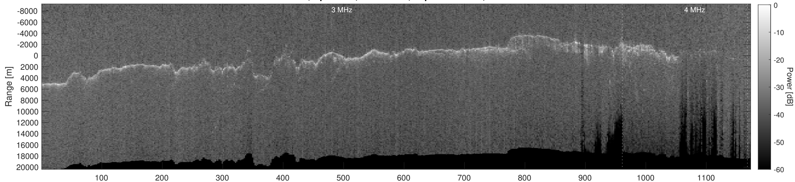
Orbit 10956, Depth-Corrected Cluttergram
