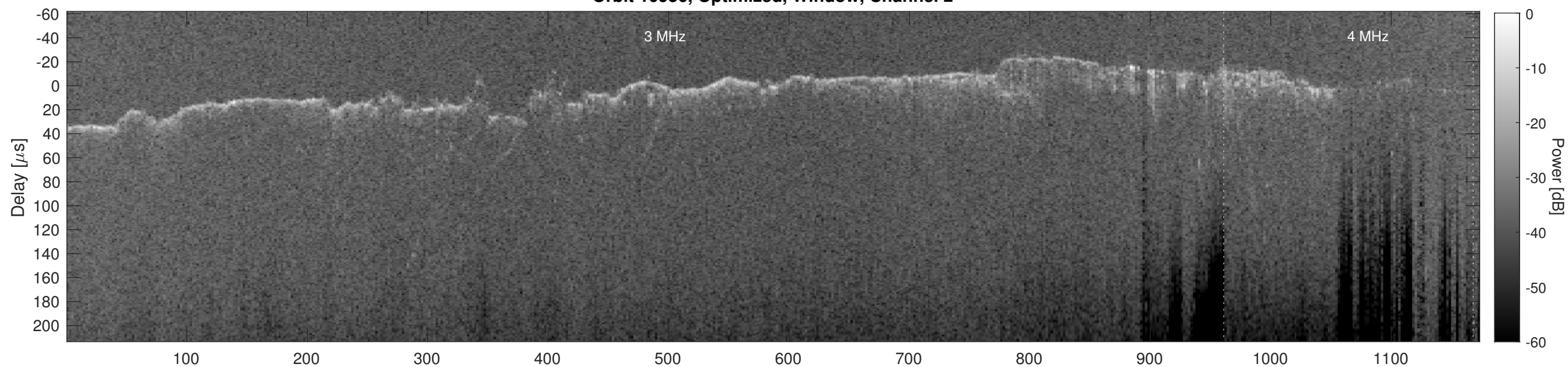
Orbit 10956, Cluttergram
