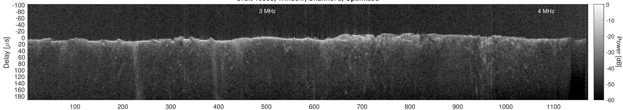
Orbit 10958, Cluttergram
