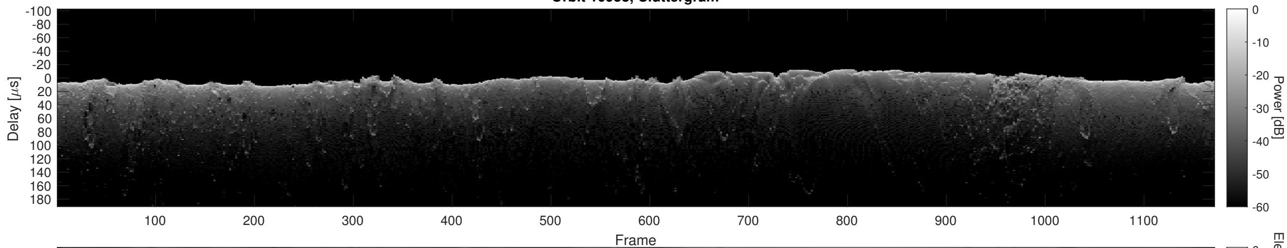
Orbit 10958, Cluttergram
