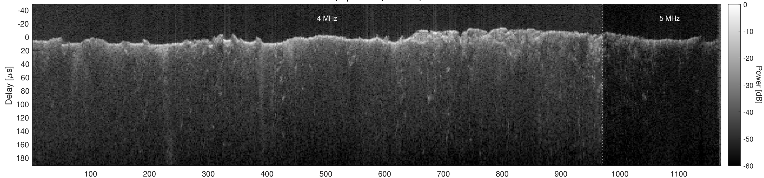
Orbit 10958, Optimized, Window, Channel 2
