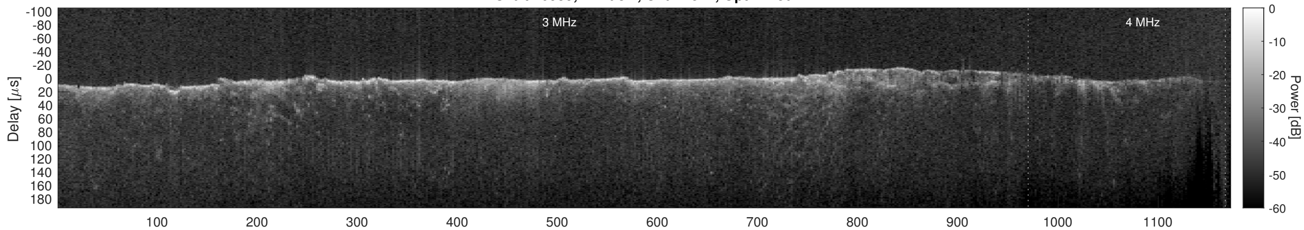
Orbit 10959, Cluttergram
