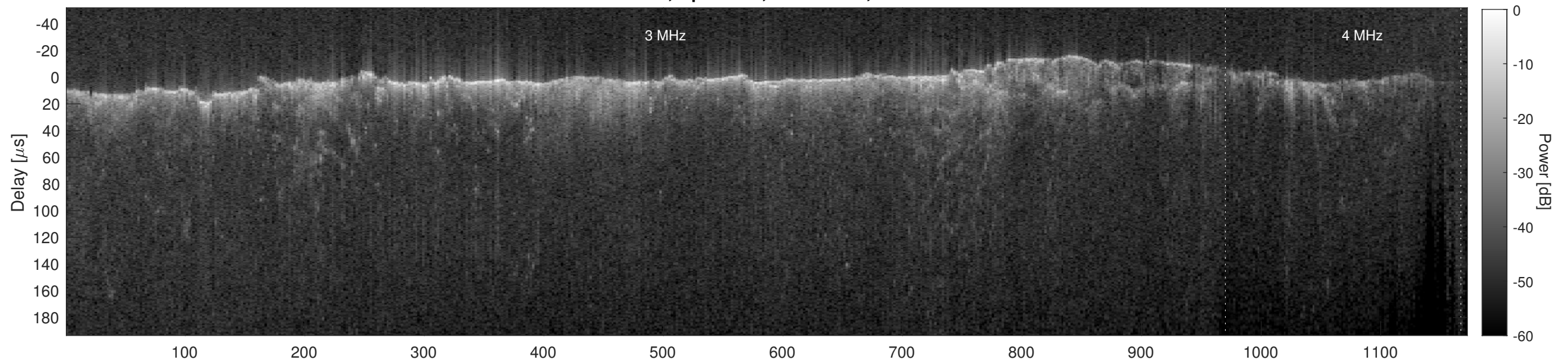
Orbit 10959, Cluttergram
