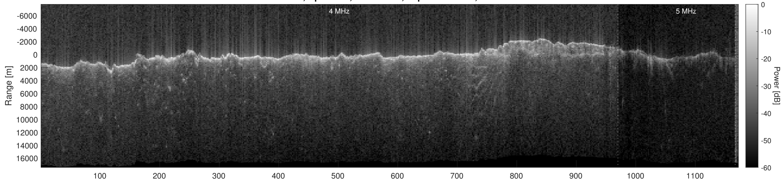
Orbit 10959, Optimized, No Window, Depth-Corrected, Channel 2
