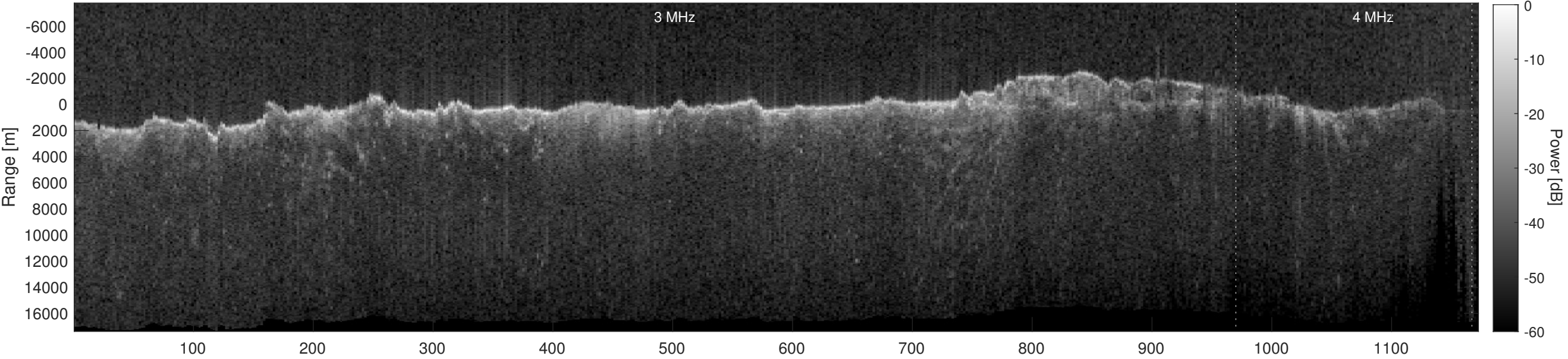
Orbit 10959, Depth-Corrected Cluttergram
