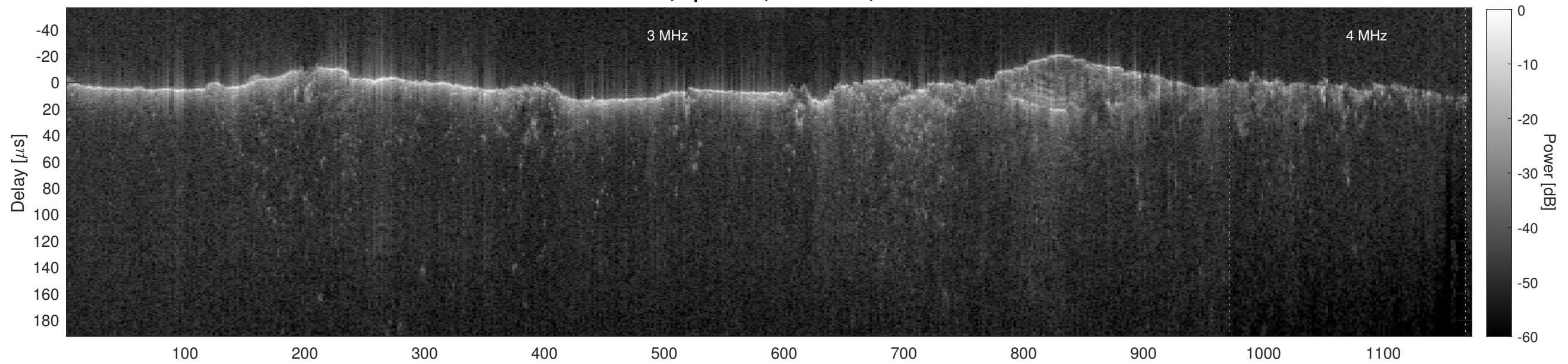
Orbit 10960, Cluttergram
