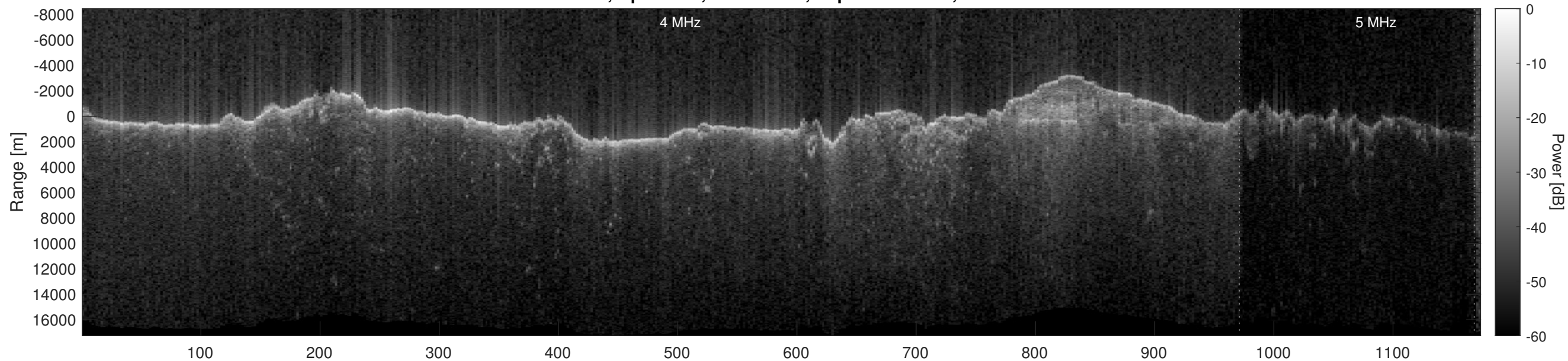
Orbit 10960, Optimized, No Window, Depth-Corrected, Channel 2
