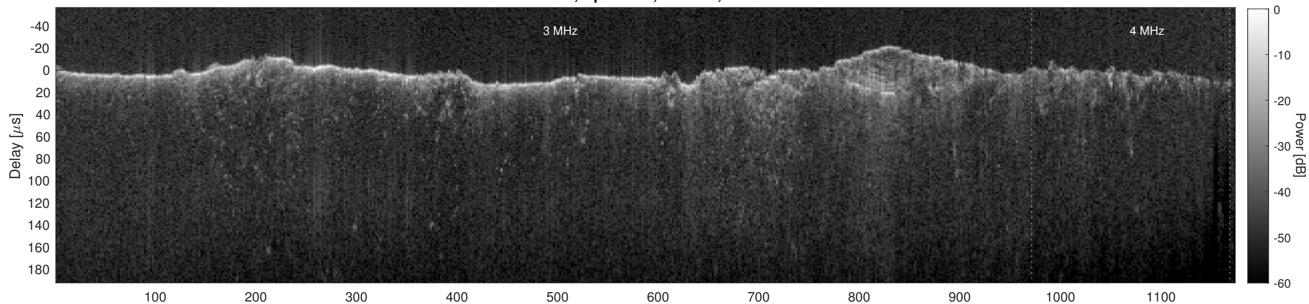
Orbit 10960, Cluttergram
