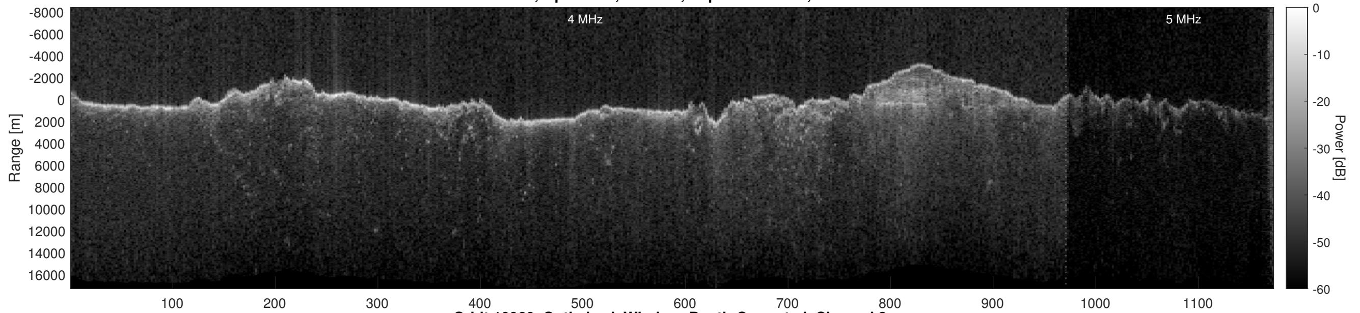
Orbit 10960, Optimized, Window, Depth-Corrected, Channel 2
