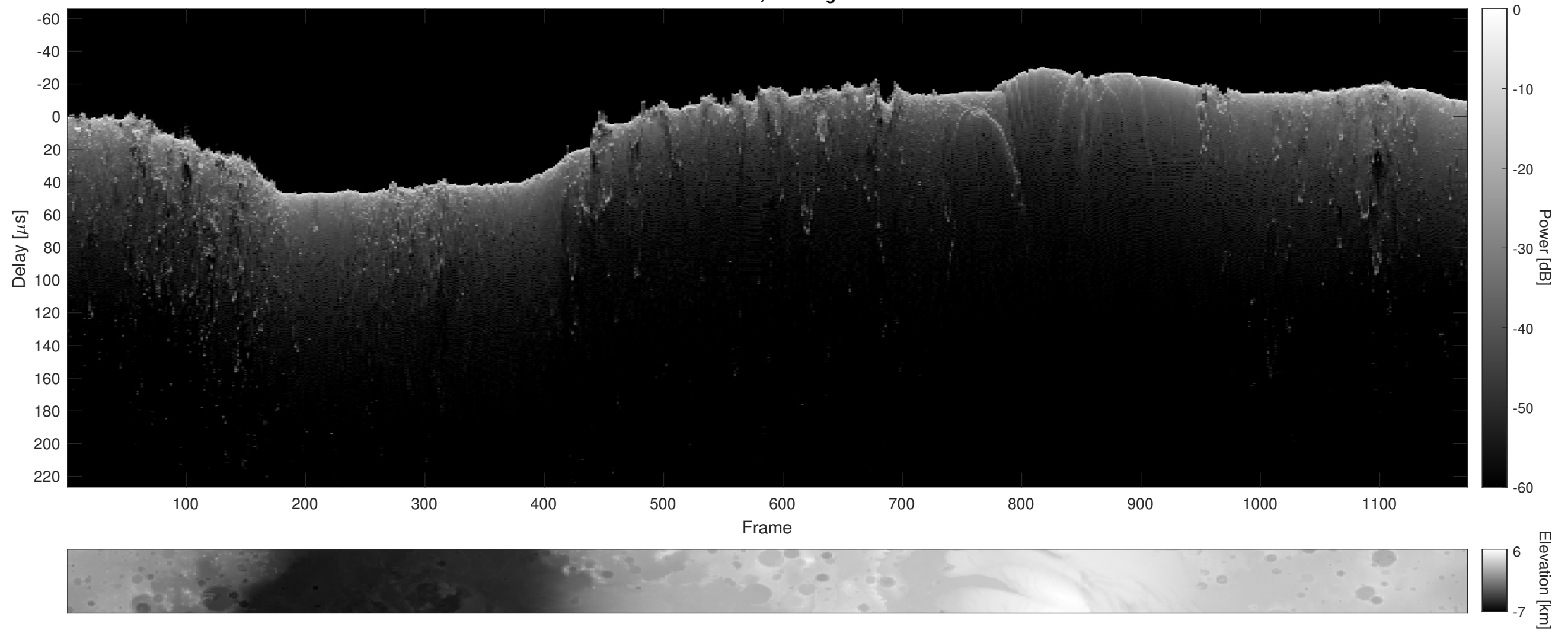
Orbit 10962, Cluttergram
