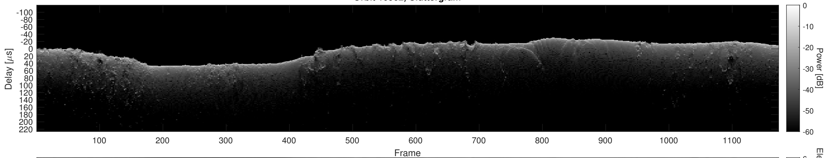
Orbit 10962, Cluttergram
