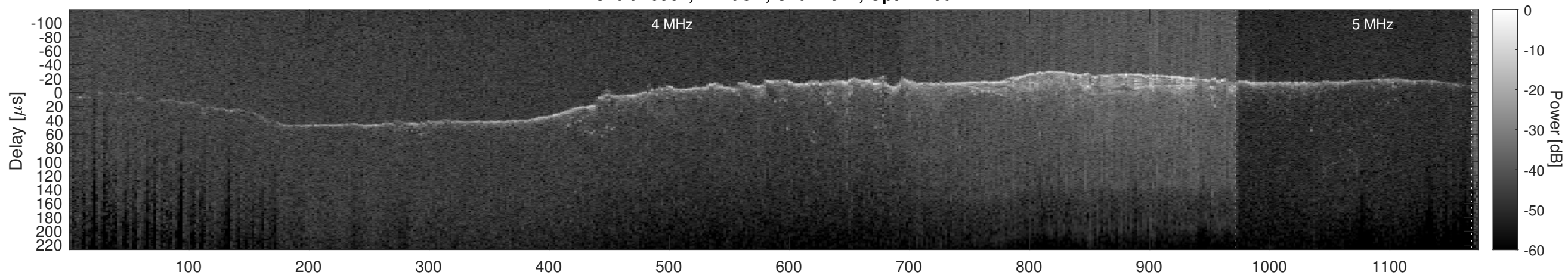
Orbit 10962, Cluttergram
