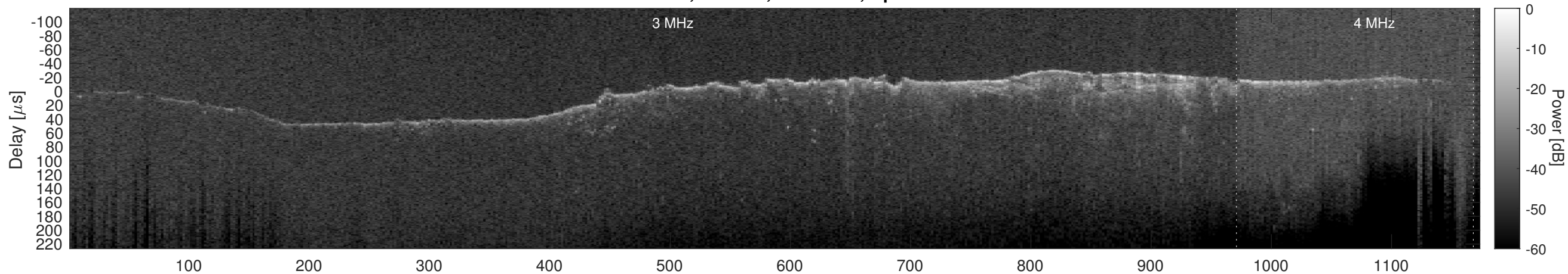
Orbit 10962, Cluttergram
