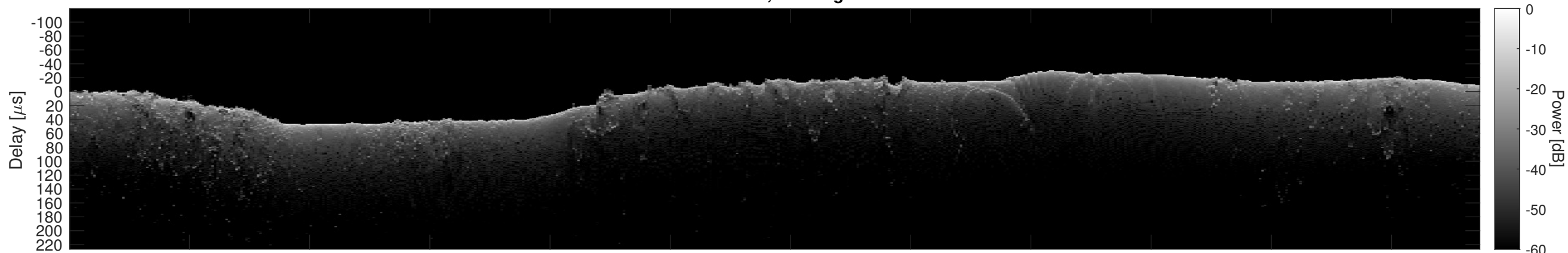
Orbit 10962, Cluttergram
