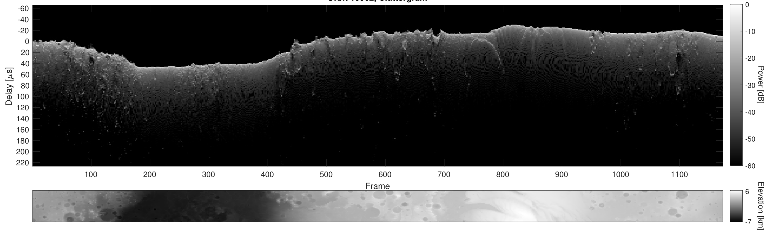
Orbit 10962, Cluttergram
