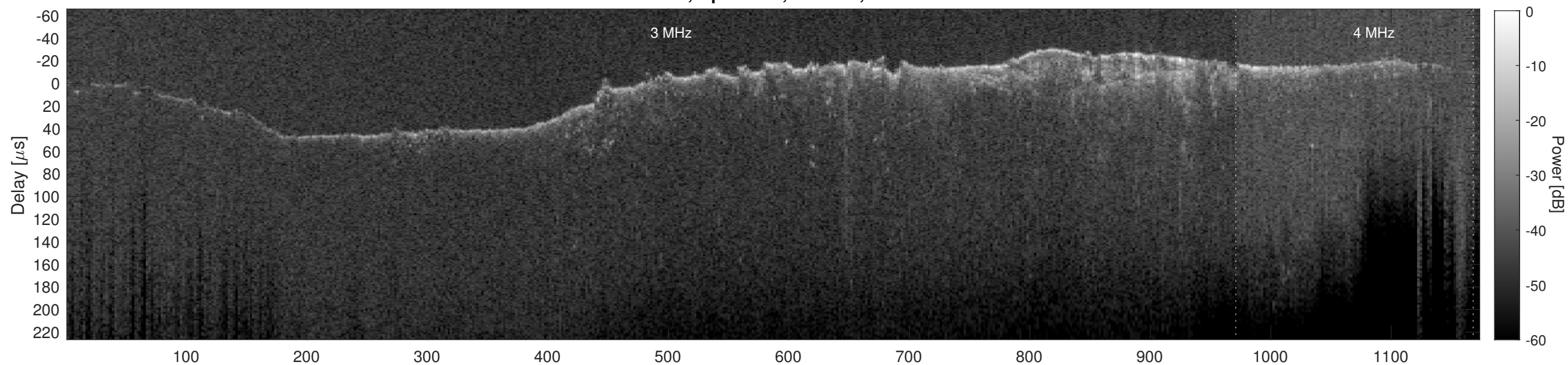
Orbit 10962, Cluttergram
