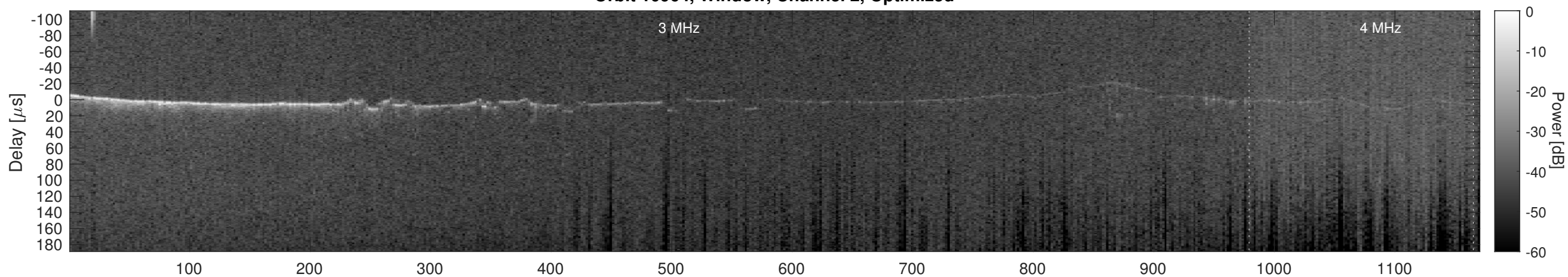
Orbit 10964, Cluttergram
