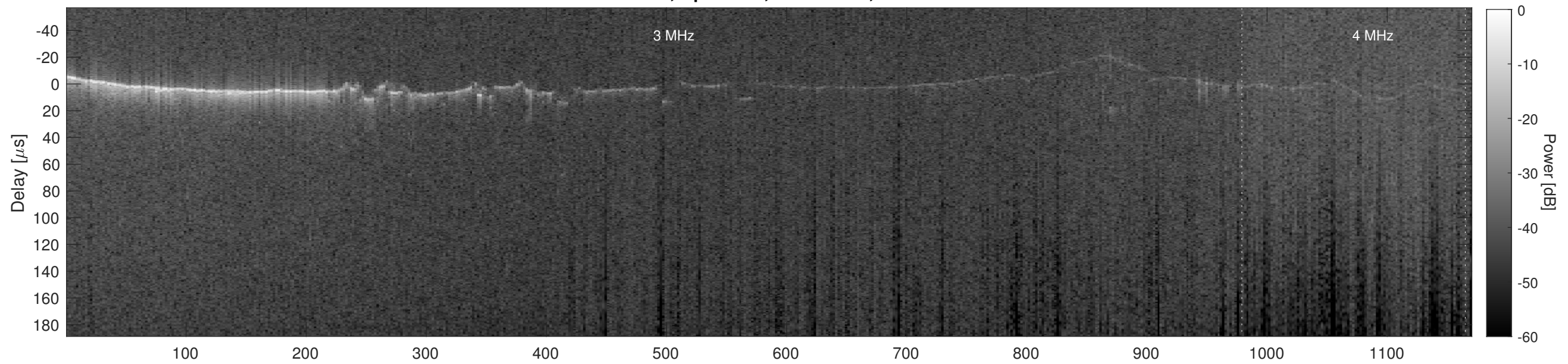
Orbit 10964, Cluttergram
