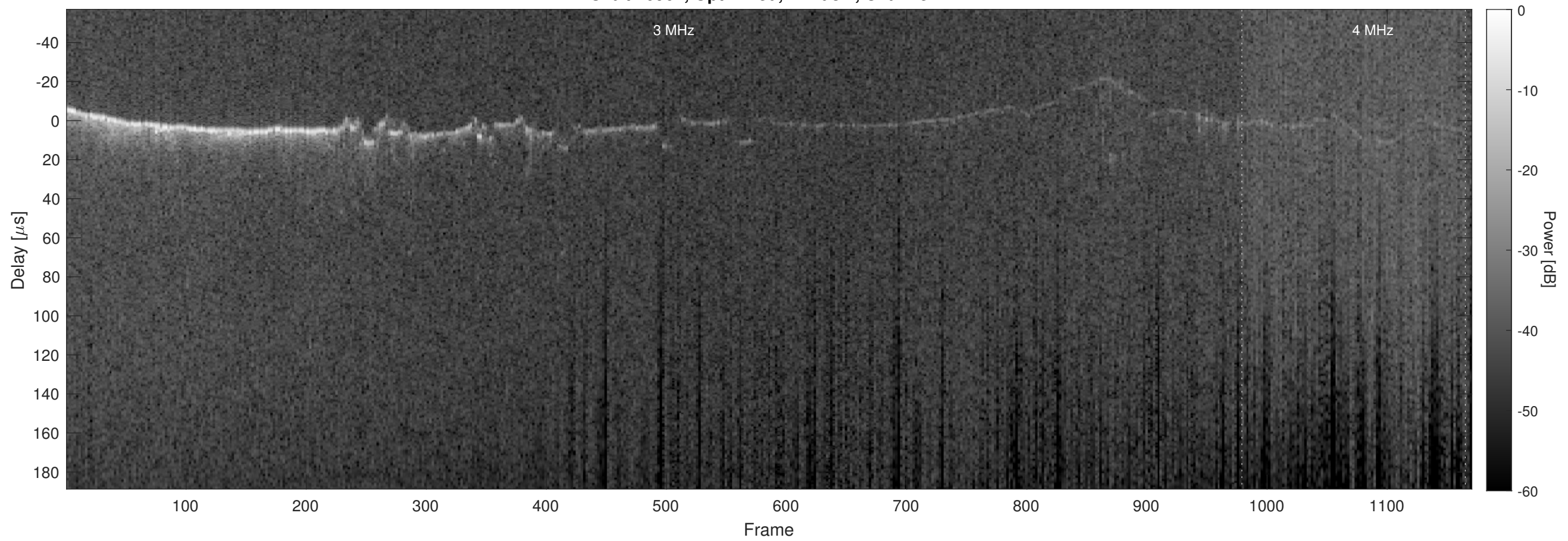
Orbit 10964, Optimized, Window, Channel 2
