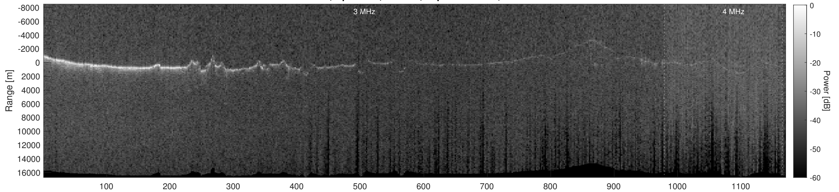
Orbit 10964, Depth-Corrected Cluttergram
