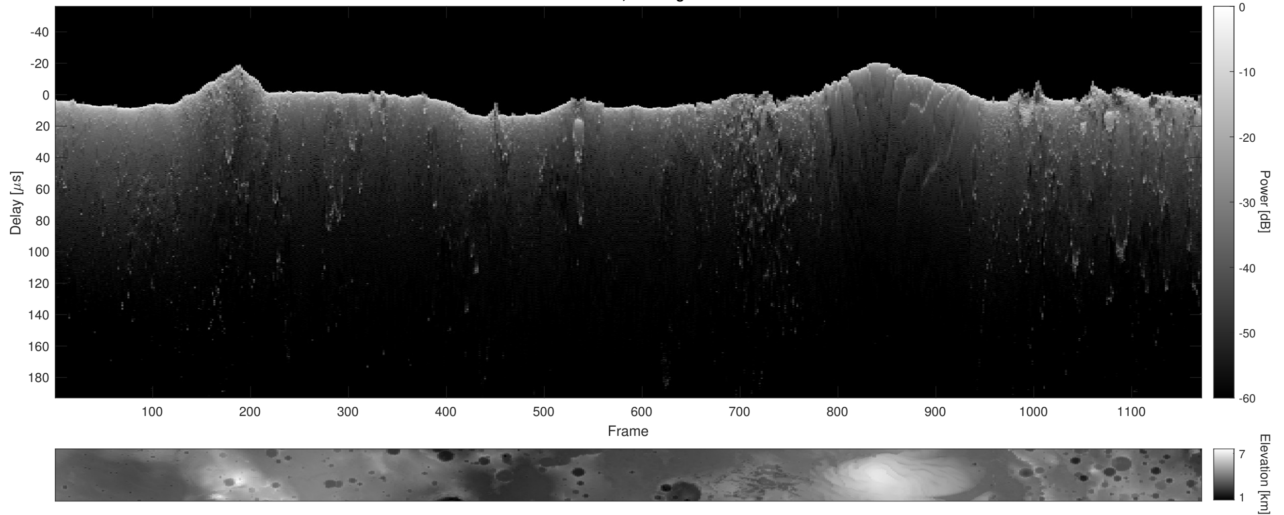
Orbit 10967, Cluttergram
