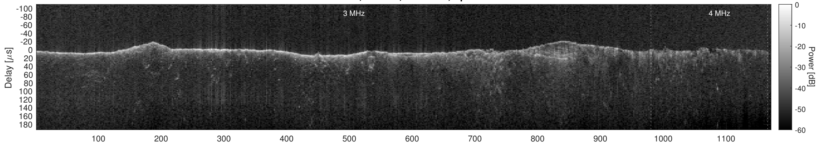
Orbit 10967, Cluttergram
