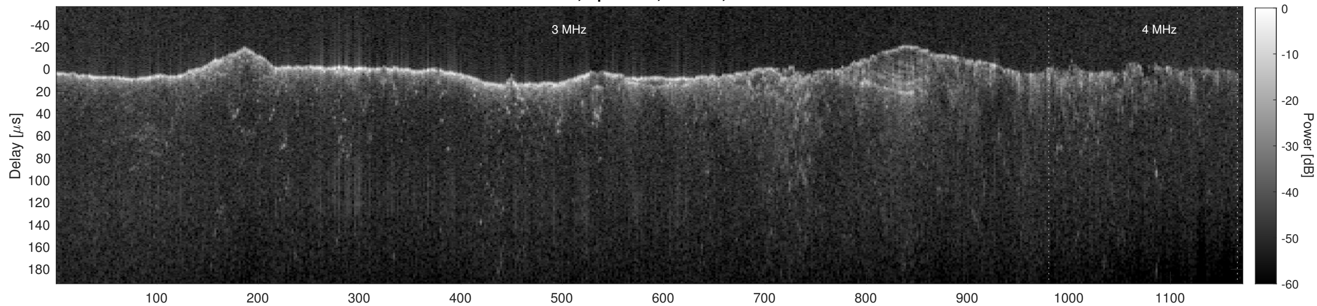
Orbit 10967, Cluttergram
