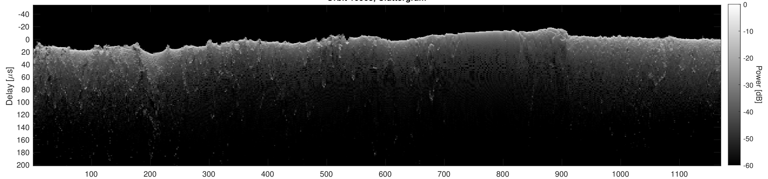
Orbit 10968, Cluttergram
